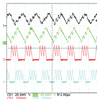
Figure 7. Output Voltage Ripple in PFM Mode
