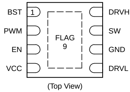
Figure 1. Pin Diagram
