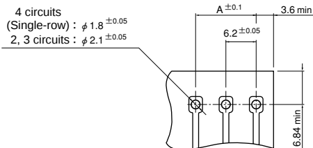
Inner-housing lock
