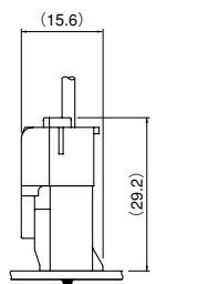
Outer-housing lock
