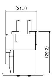
Outer-housing lock
