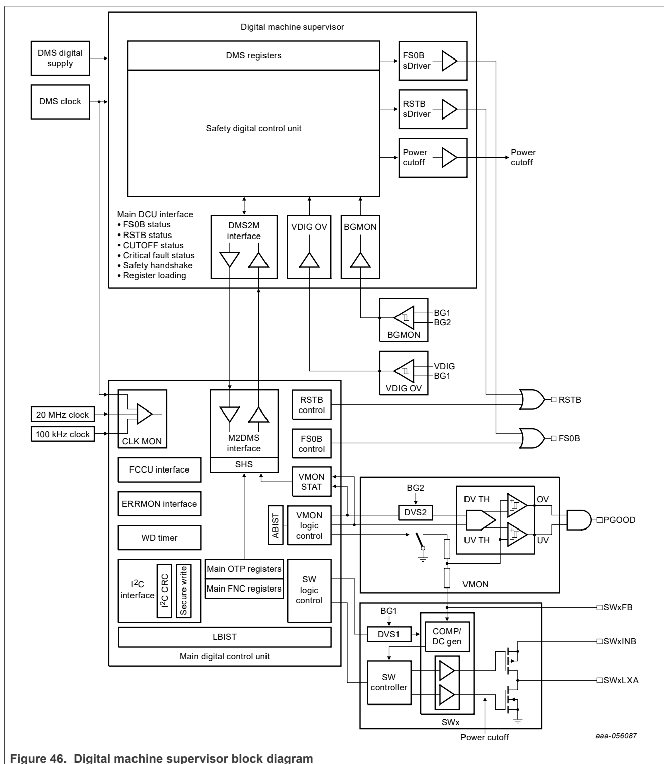
Figure 46. Digital machine supervisor block diagram
