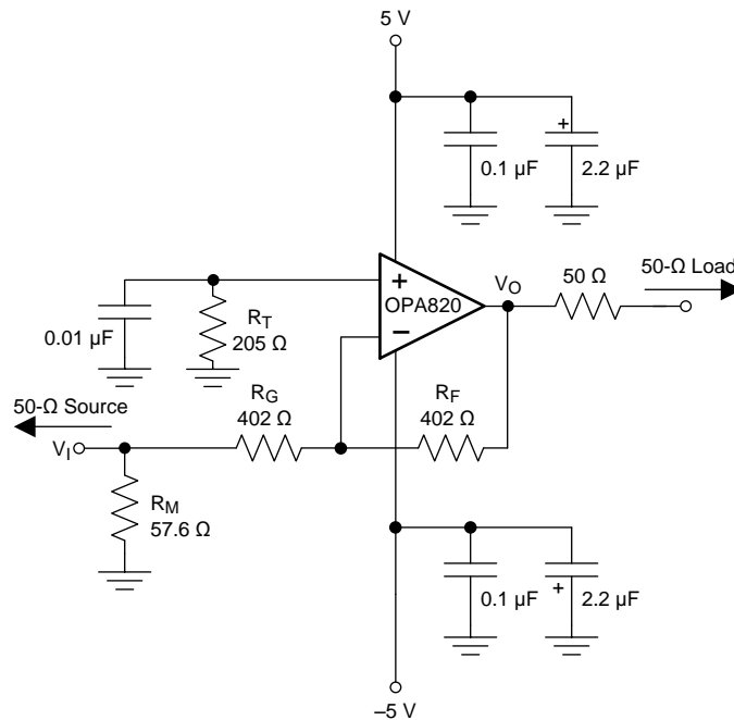
Figure 56. Inverting G = -1 Specifications and Test Circuit
