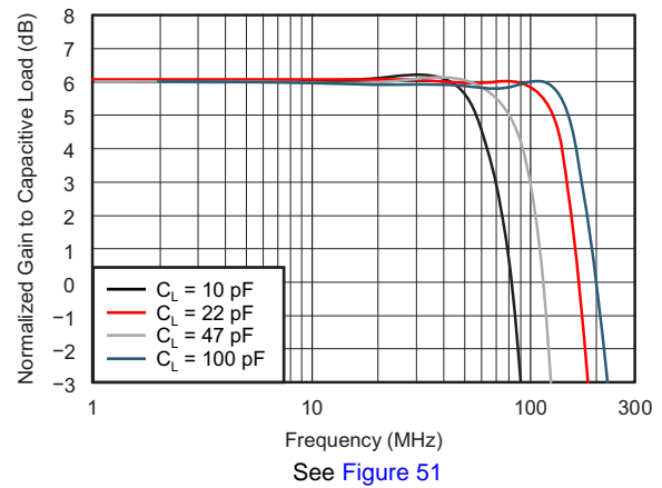
Figure 43. Frequency Response vs Capacitive Load
