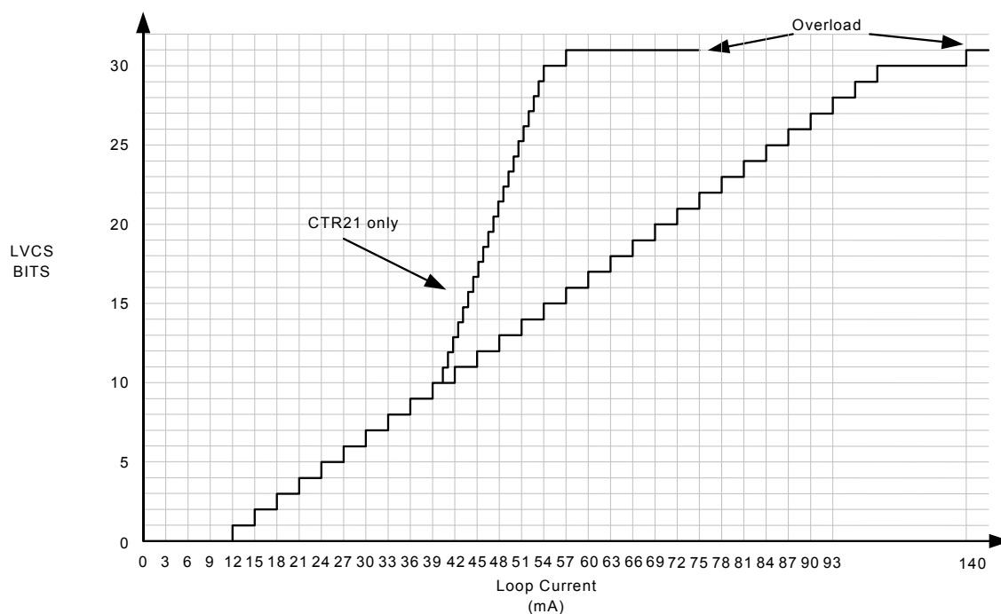
Figure 8. Loop Current
