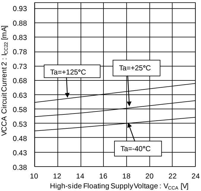
Figure 15. VCCA Circuit Current 2 vs High-side Floating Supply Voltage (OUTA=H)
