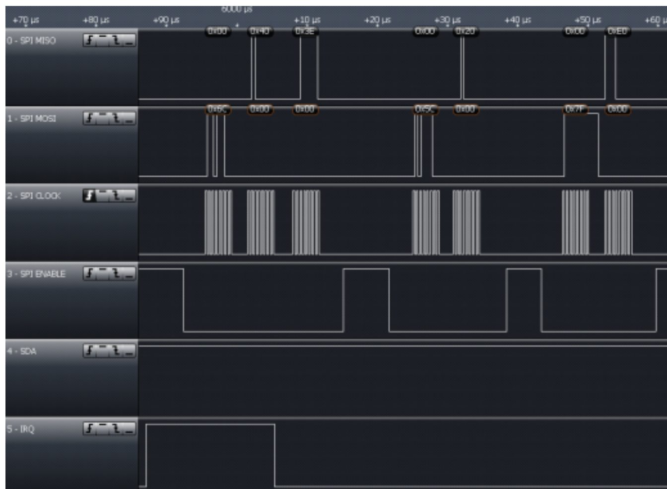
Figure 5-24. Second IRQ After Inventory Command
