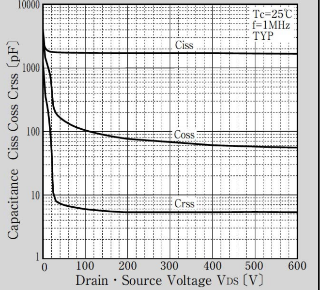
Capacitance Characteristics
