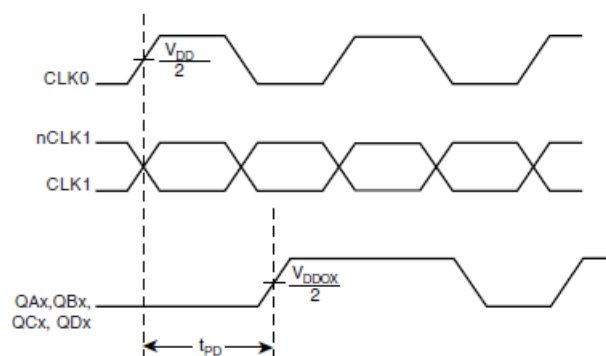
PROPAGATION DELAY
