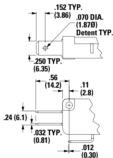
4A 0.250" Quick Connect
