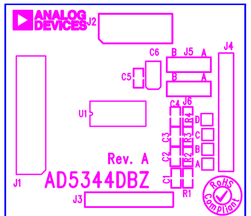
Figure 14. EVAL-AD5344DBZ Daughter Board Component Placement
