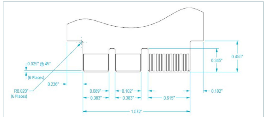
Figure 8 Edge connector details
