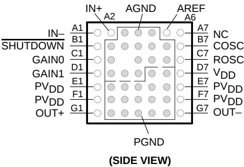
MicroStar Junior™ (GQC) Package (TOP VIEW)
