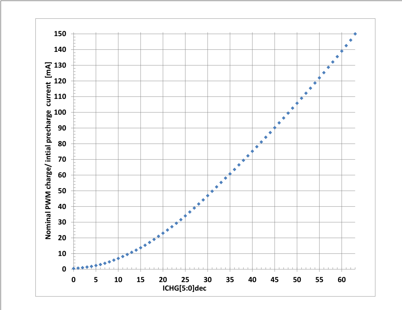
Figure 61 Configurable discharge currents in PWM operation
