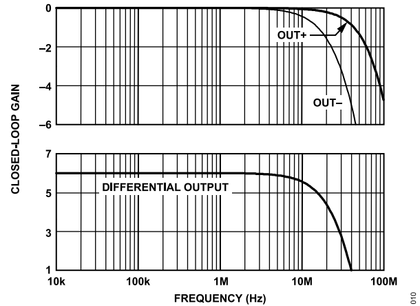
Figure 48. Closed-Loop AC Gain (Differential Outputs)
