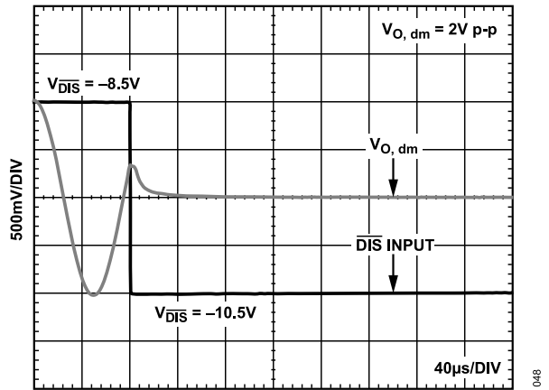
Figure 39. Disable Turn-Off Time
