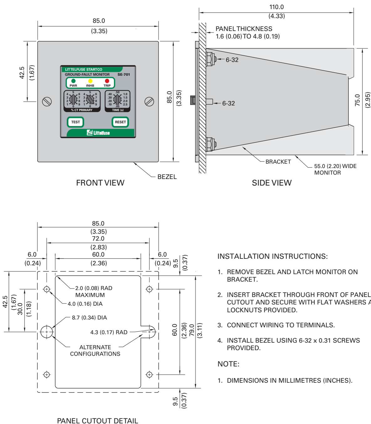
FIGURE 9. PMA-55 Panel-Mount Adapter.
