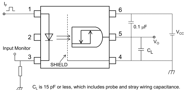
Fig. 13.1.7 Switching Time Test Circuit and Waveform
