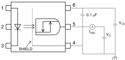
Fig. 13.1.5 I_{OL} Test Circuit
