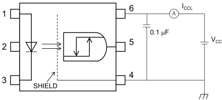
Fig. 13.1.3 I_{CCL} Test Circuit
