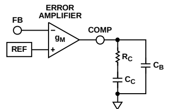
Figure 24. Compensation Components
