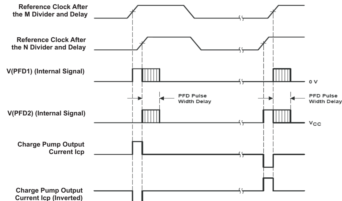
Figure 25. Charge Pump
