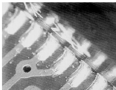
Picture 5. Good solder joint.
