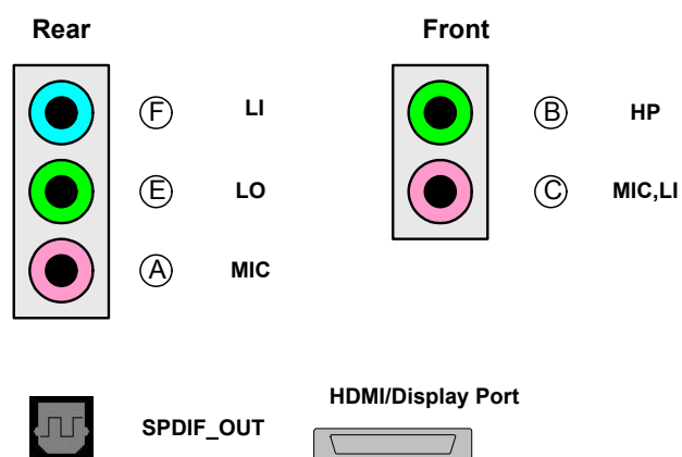
Figure 21. Port Configurations
