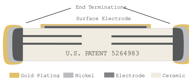
Sectional Diagram: Sizes L18 & L41
