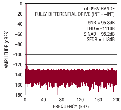
Figure 6c. IN^+/IN^- = -1\text{dBFS} 2kHz Fully Differential Sine, Common Mode = 2.5V, 32k Point FFT, f_{\text{SAMPL}} = 400\text{kps} . Circuit Shown in Figure 6a with LT6237 Amplifiers, R_{\text{FILT}} = 24.9\Omega , C_{\text{FILT}} = 1\text{nF}
