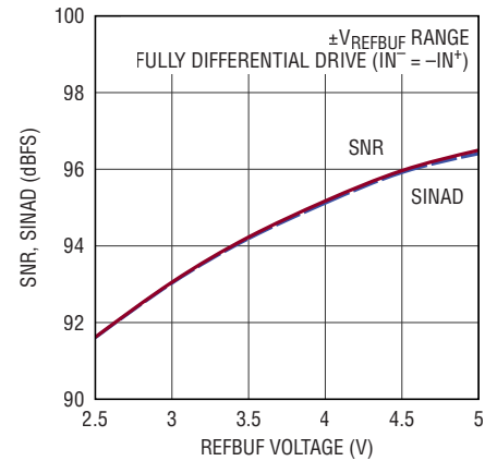
SNR, SINAD vs V_{REFBUF} , f_{IN} = 2\text{kHz}
