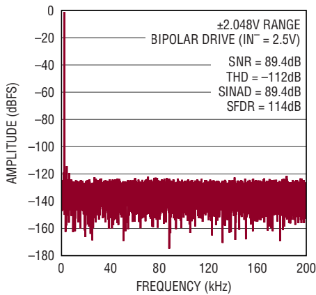
Figure 6d. IN^+ = -1\text{dBFS} 2kHz Bipolar Sine, IN^- = 2.5\text{V} , 32k Point FFT, f_{\text{SAMPL}} = 400\text{kps} . Circuit Shown in Figure 6a with LT6237 Amplifiers, R_{\text{FILT}} = 24.9\Omega , C_{\text{FILT}} = 1\text{nF}
