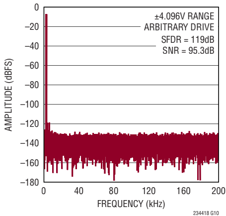
32k Point Arbitrary Two-Tone FFT f_{SAMPL} = 400\text{kHz} , IN^+ = -7\text{dBFS} 2kHz Sine, IN^- = -7\text{dBFS} 3.1kHz Sine
