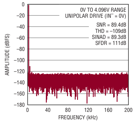
Figure 6e. IN^+ = -1\text{dBFS} 2kHz Unipolar Sine, IN^- = 0\text{V} , 32k Point FFT, f_{\text{SAMPL}} = 400\text{kps} . Circuit Shown in Figure 6a with LT6237 Amplifiers, R_{\text{FILT}} = 24.9\Omega , C_{\text{FILT}} = 1\text{nF}
