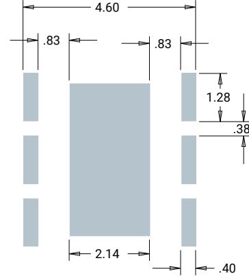
Recommended Stencil Openings*
