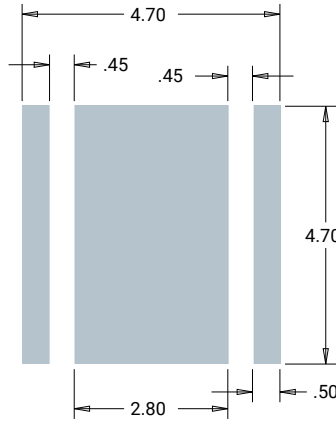
Recommended Solder Pad (Solder Mask Pattern)
