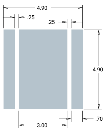
Recommended Copper Layout
