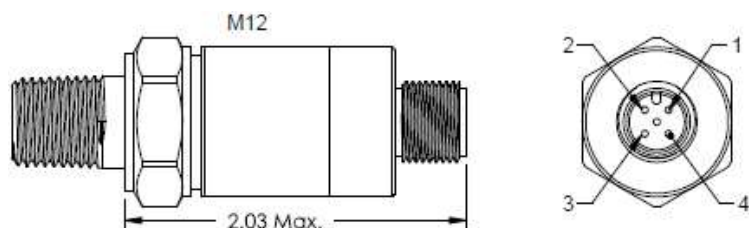
Voltage Output Wiring
