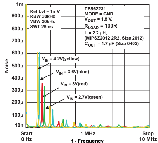
Figure 42. Spurious Output Noise, 100R Load – TPS62231
