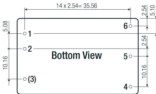
Pin Connections with suffix /P
