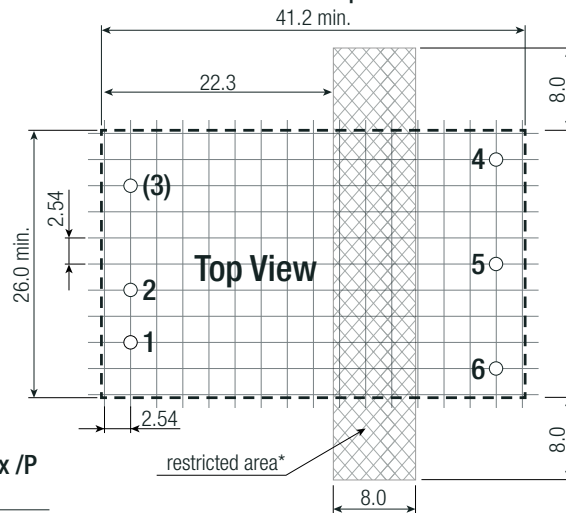
Recommended Footprint Details
