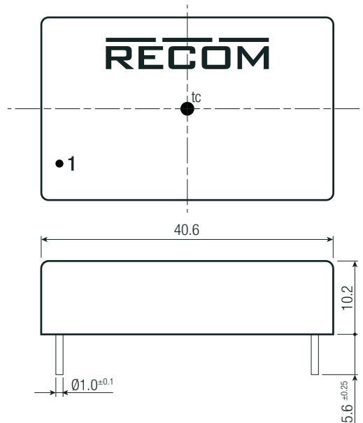
Dimension Drawing (mm)
