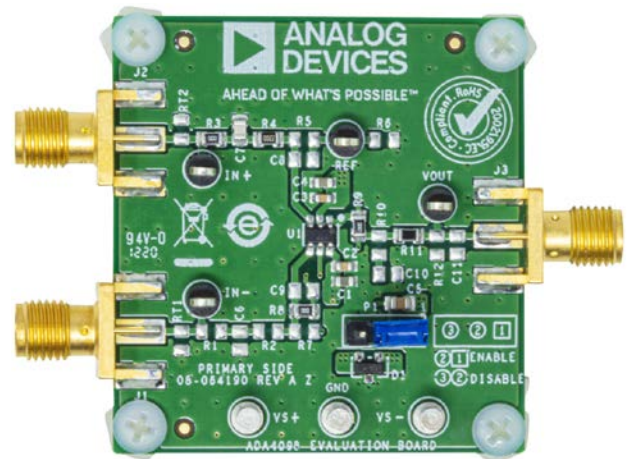
Figure 1. EVAL-ADA4098-1HUIZ, Primary Side
