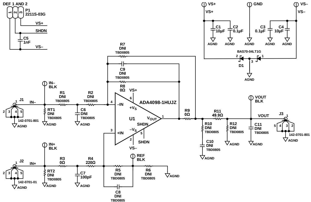
Figure 3. EVAL-ADA4098-1HUJZ Schematic
