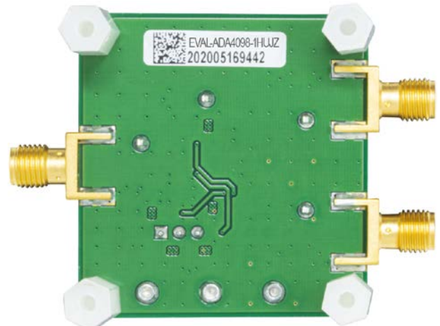
Figure 2. EVAL-ADA4098-1HUIZ, Secondary Side
