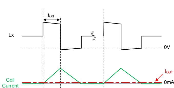
The PWM/PFM control (MODE="L") : Example of light load operation
