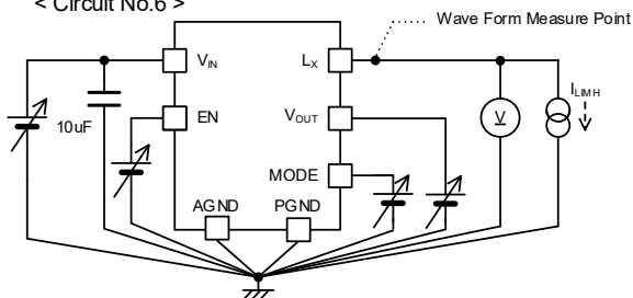
< Circuit No.6 >
