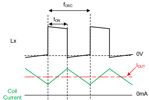
The PWM/PFM control (MODE="L") : Example of heavy load operation
