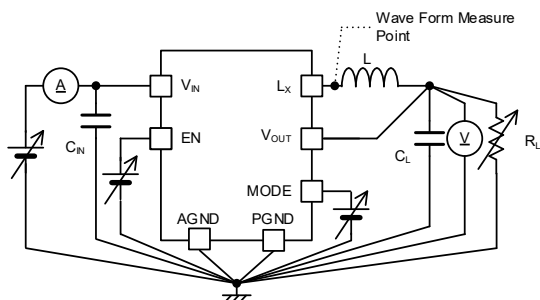
< Circuit No.1 >
