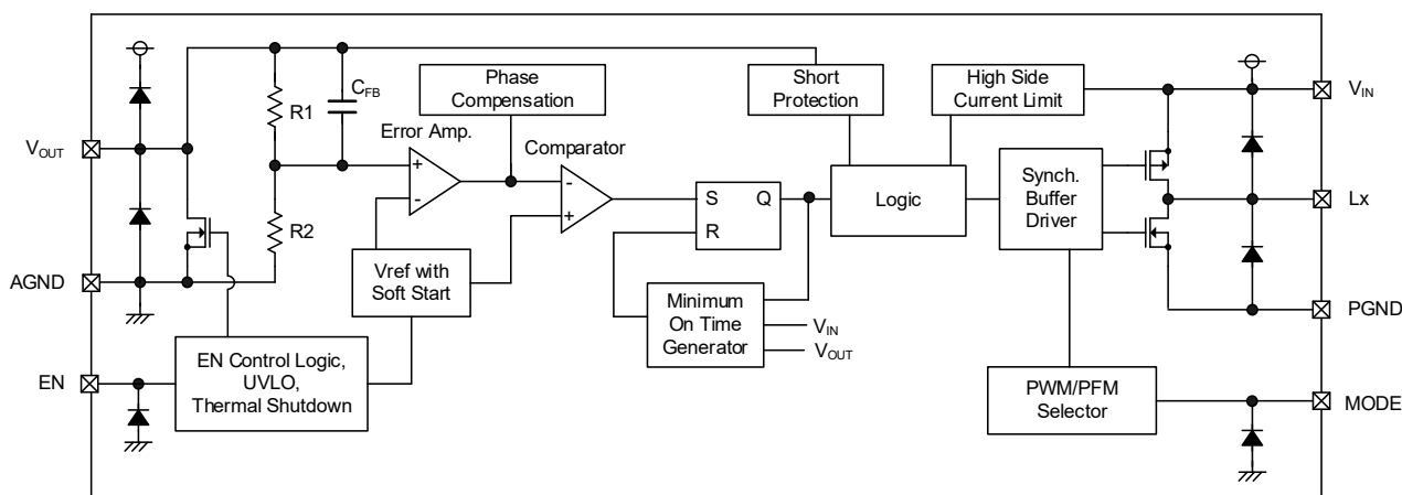
BLOCK DIAGRAM (BType)
