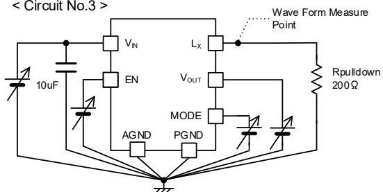
< Circuit No.3 >
