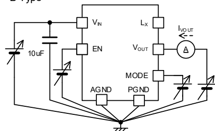
< Circuit No.7 >
