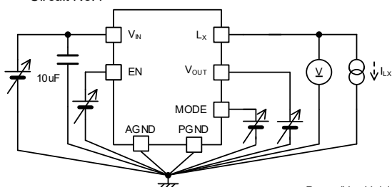
< Circuit No.4 >
