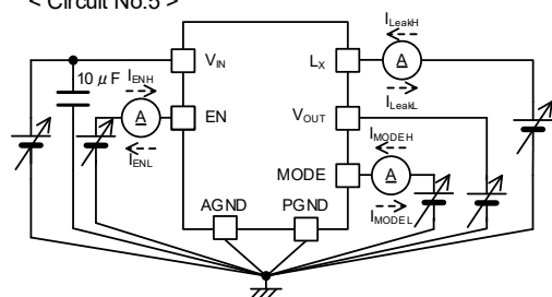
< Circuit No.5 >
