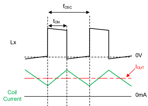
The PWM control (MODE="H") : Example of heavy load operation
