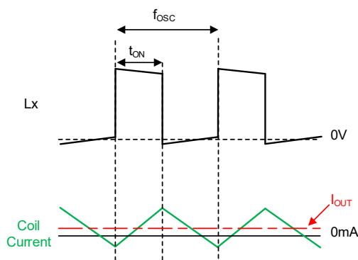
The PWM control (MODE="H") : Example of light load operation
