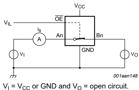
Fig. 6. Test circuit for measuring ON-state leakage current (one switch)
