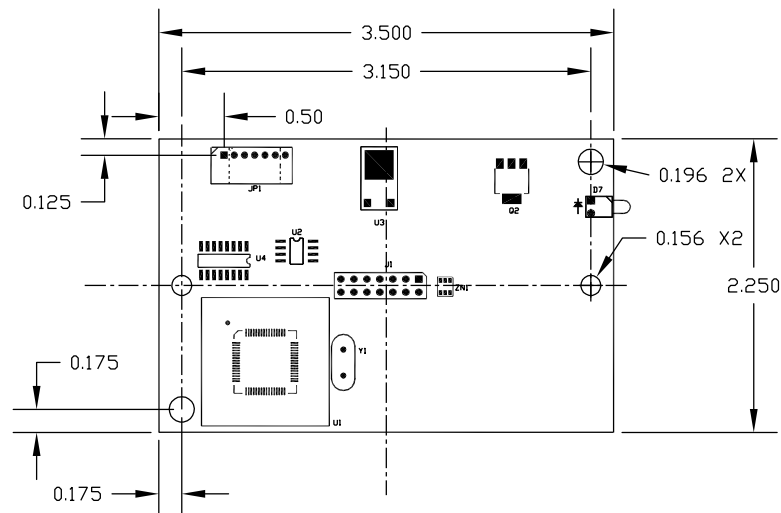
Figure 1. EX II 17xxSC Overall Dimensions
