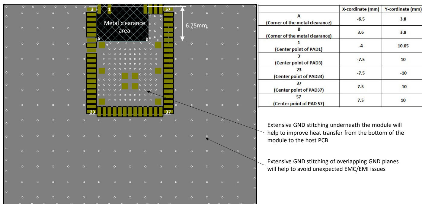
Figure 8.18. Application Layout of SiWN917Y1GA
