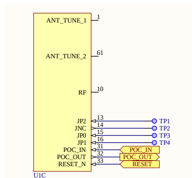
Figure 8.9. RF, Debug, and Reset Connection
