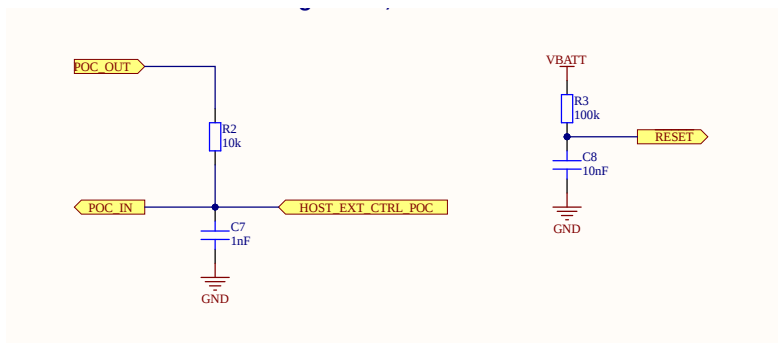
Figure 8.11. Reset Configuration
