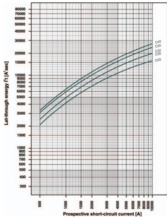
Characteristic C (40A), 240V
