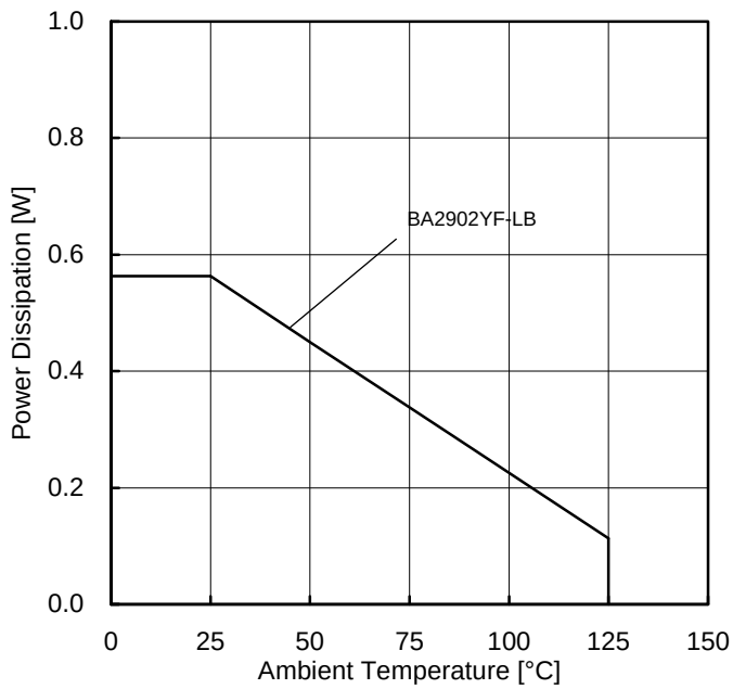
Figure 26. Derating Curve
