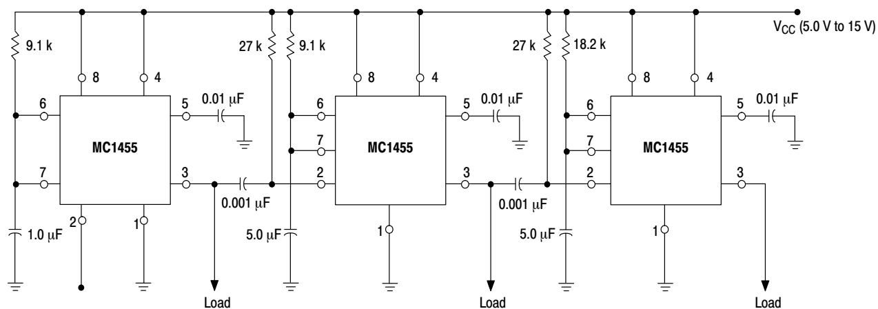
Figure 26. Sequential Timer
