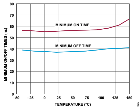
Figure 25. Bottom Switch Minimum On/Off Times vs Temperature
