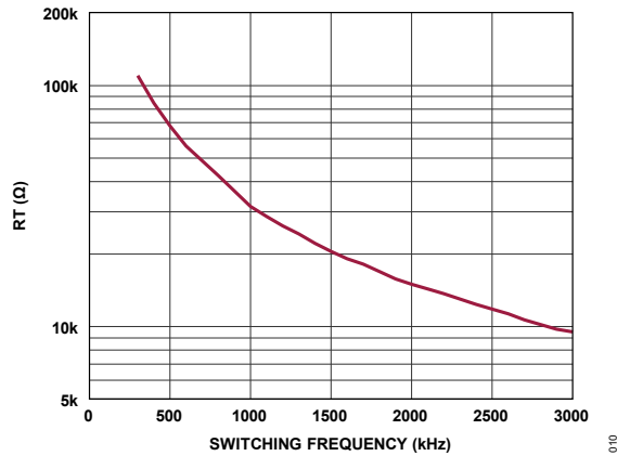
Figure 10. RT Value vs Switching Frequency
