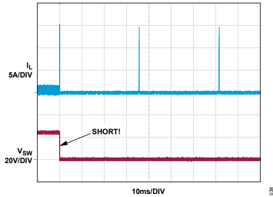
Figure 38. Hiccup during Output Short Circuit. See Figure 1 , V_{IN} = 9V .
