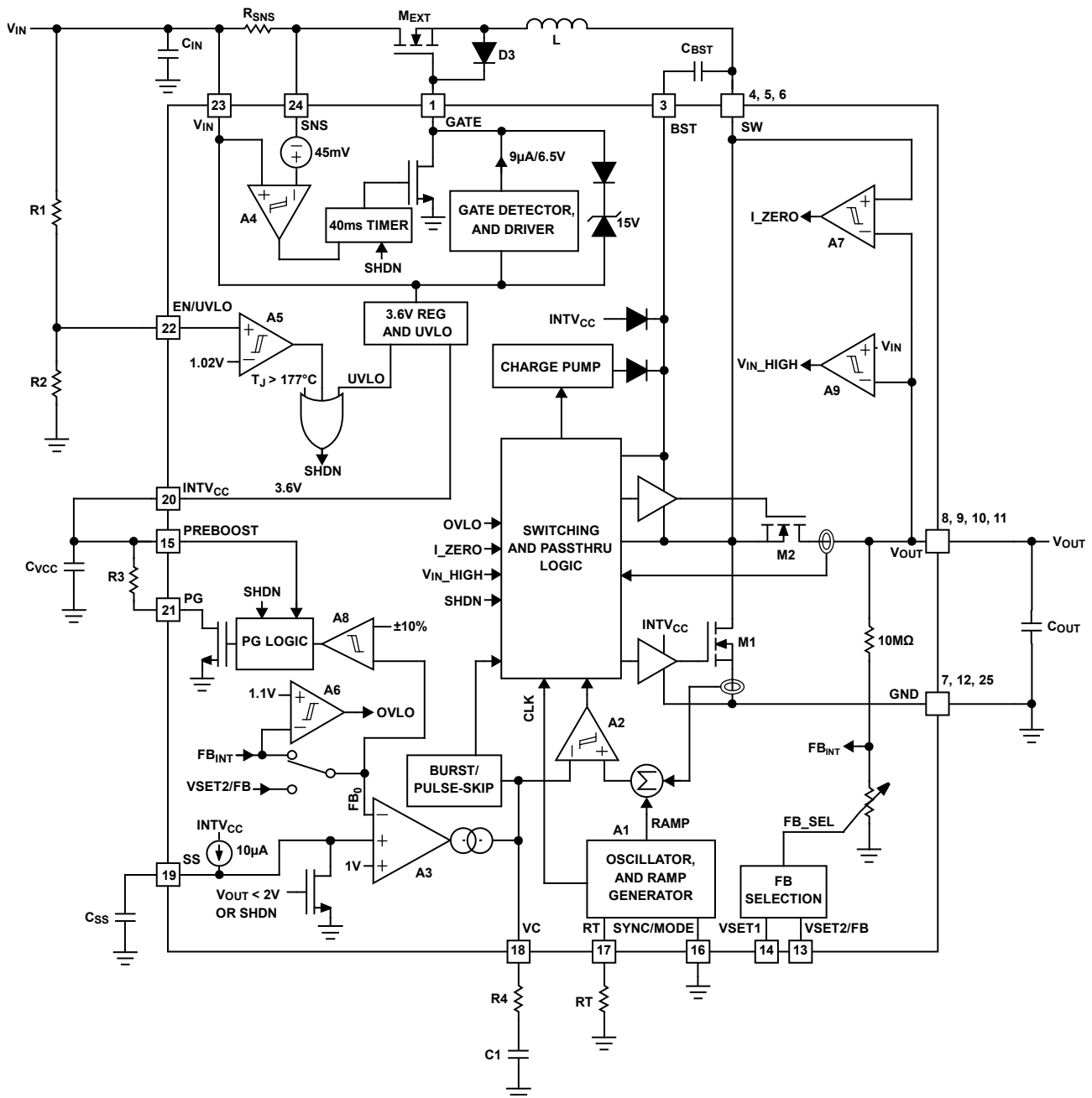
Figure 41. Block Diagram
