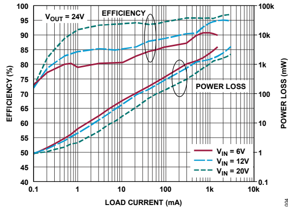
Figure 4. Burst Mode Efficiency and Power Loss vs Output Current. See Figure 1 with SYNC/MODE = 0V.
