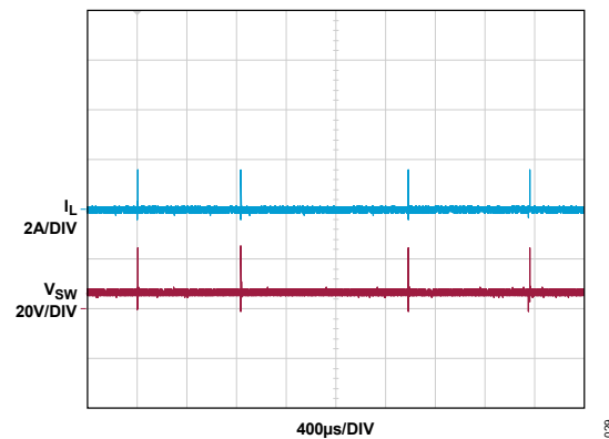
Figure 29. Light Load Low I_Q Burst Mode Operation. See Figure 1, SYNC/MODE = 0V , V_{IN} = 6V , I_{LOAD} = 0A
