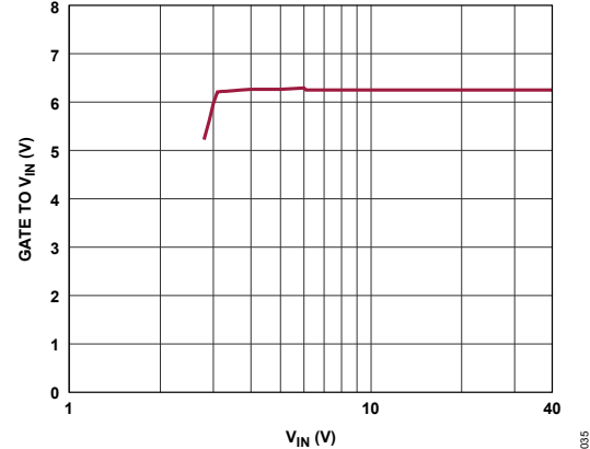
Figure 35. GATE to VIN Regulation Voltage vs V_{IN}
