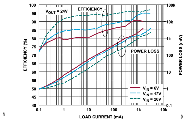
Figure 2. Efficiency and Power Loss vs Load Current in Burst Mode (SYNC/MODE = 0V)
