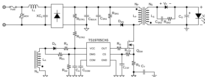
Flyback Converter
