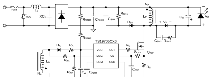
Buck-Boost Converter
