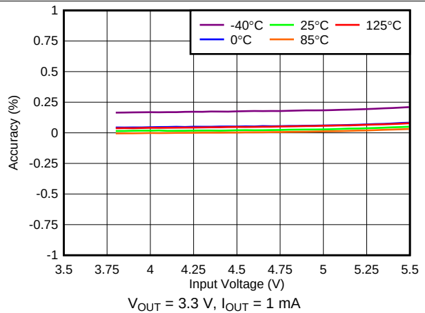
Figure 16. 3.3 V Regulation vs V_{IN} (Line Regulation)
