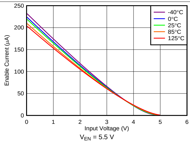
Figure 24. I_{EN} vs V_{IN}
