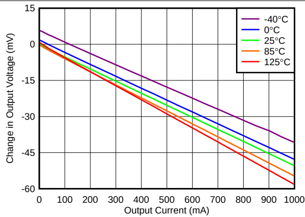
Figure 13. Load Regulation vs I_{OUT}
