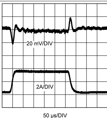
V_{IN} = 5.0\text{ V} , V_{OUT} = 2.5\text{ V} , I_{OUT} = 0.4\text{-A} to 3.6\text{-A} to 0.4\text{-A} Step 20 mV/DIV, 20-MHz Bandwidth Limited Refer to Table 5 for BOM, includes optional components
