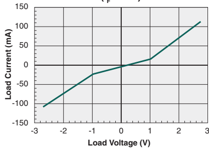
Typical Load Current vs. Load Voltage ( I_F=5\text{mA} )
