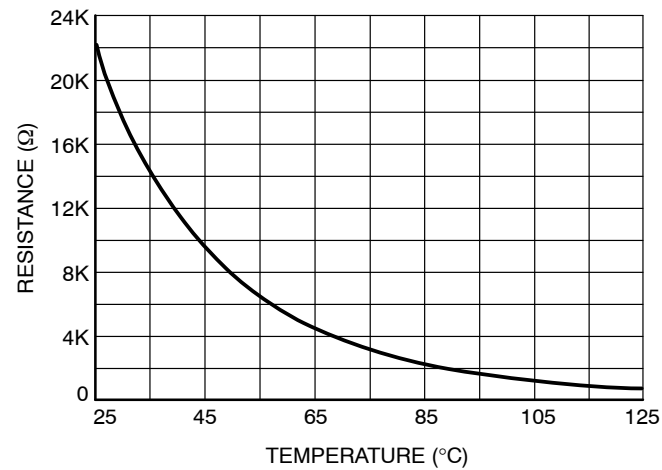
Figure 21. Thermistor Characteristic
