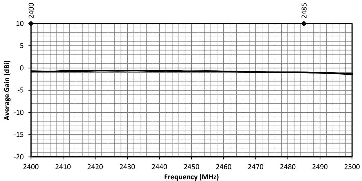
Figure 5. ANT-2.4-FPC-SH Antenna Average Gain
