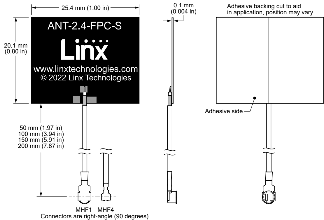
Figure 1. ANT-2.4-FPC-SH Series Antenna Dimensions
