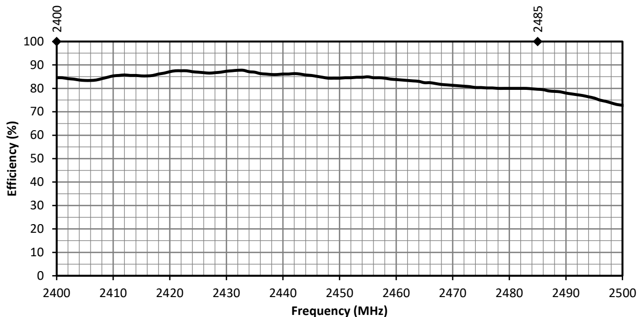
Figure 6. ANT-2.4-FPC-SH Antenna Radiation Efficiency
