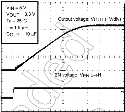
Startup Characteristics (CSS = 0.1 μF)
