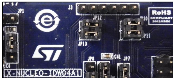
Figure 4: SPI jumper configuration
