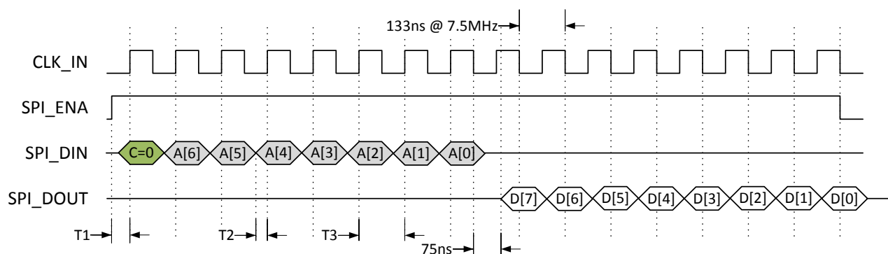
Figure 12: SPI Read timing
