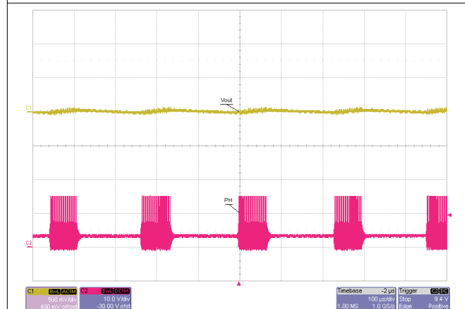
Figure 21. Eco-mode
