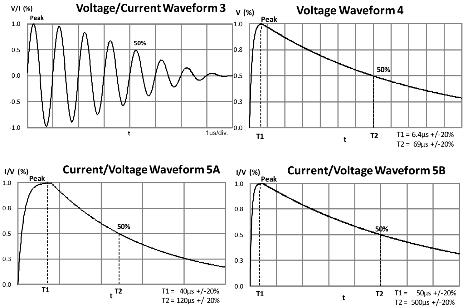
Figure 8. Lightning Waveforms
