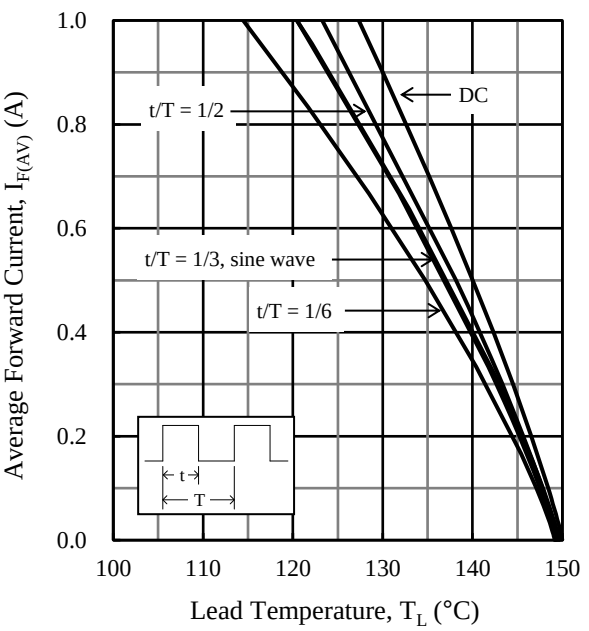
Figure 3. I_{F(AV)} vs. T_L ( T_J = 150 °C, V_R = 500 V)
