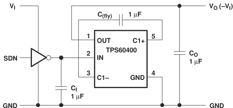
Figure 9-10. Shutdown Control
